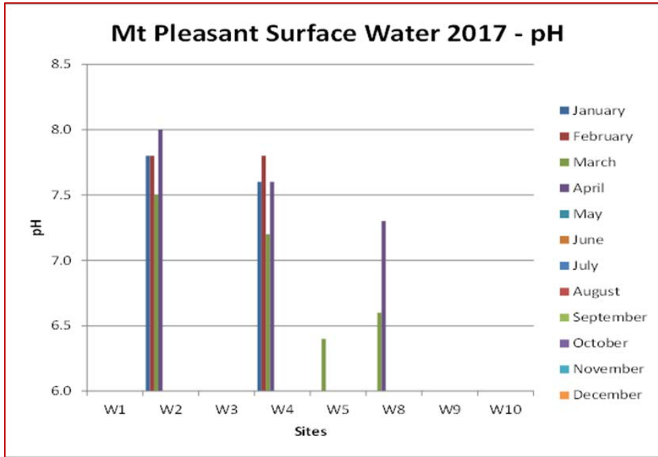
Figure 6-1 – MPO Surface Water pH
