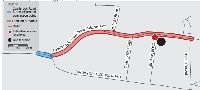
FIGURE 1 - General arrangement Dorset Road and Castlerock Road works.
