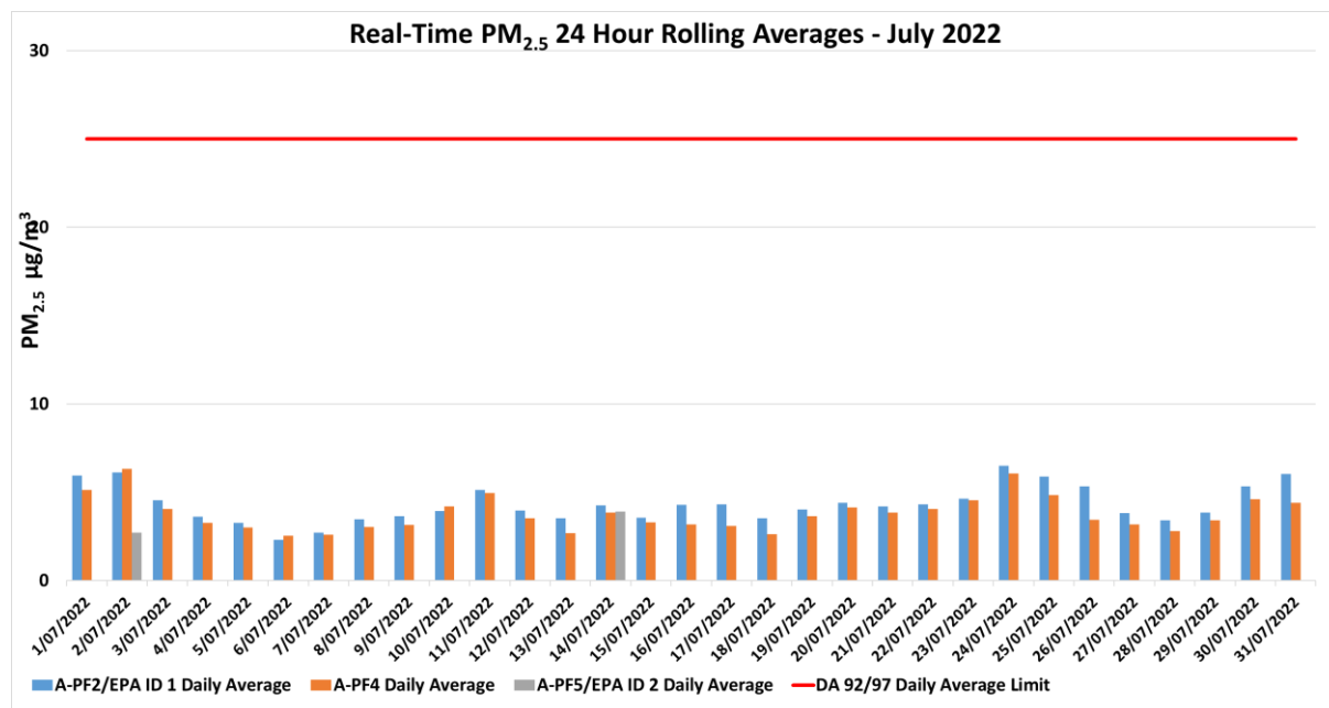
Figure 6-3: Real-time PM 2.5 24 hour rolling average results for July 2022.
