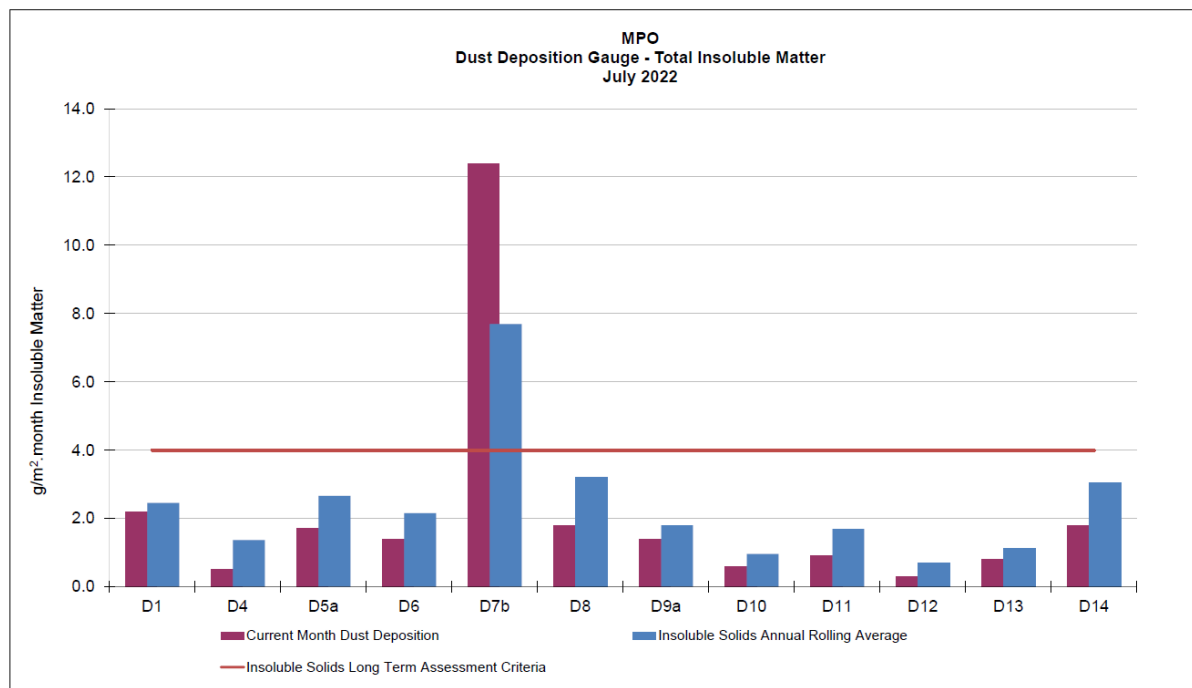
Figure 4-1: MPO Dust Deposition Monthly Results and Annual Rolling Average – July 2022
