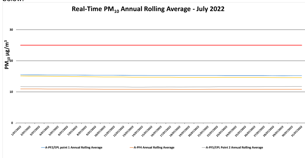
Figure 6-2: Real-time PM 10 Annual Rolling average results for July 2022.
