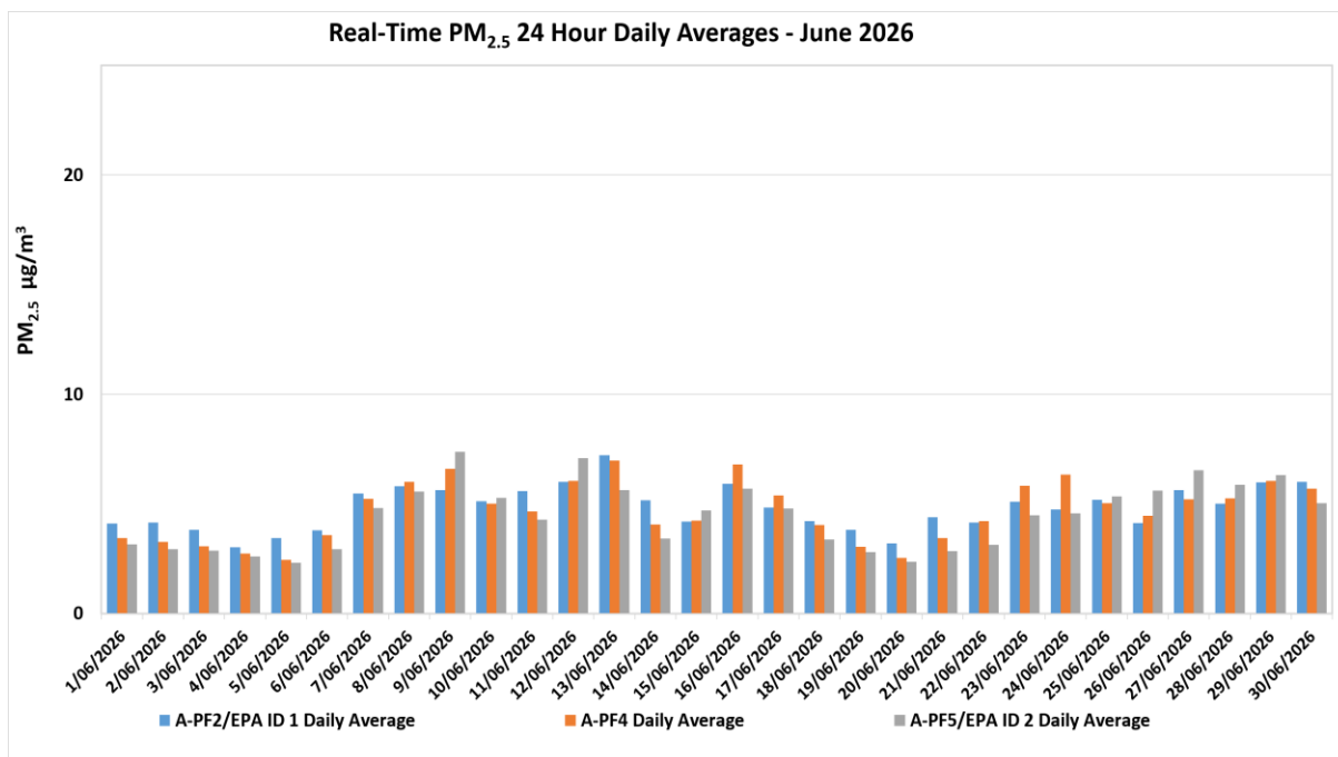
Figure 6-3: Real-time PM 2.5 24 hour Daily Average Results for June 2026.
