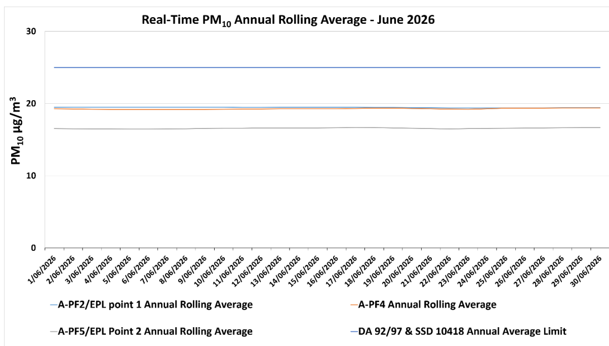
Figure 6-2: Real-time PM 10 Annual Rolling Average Results for June 2026.
