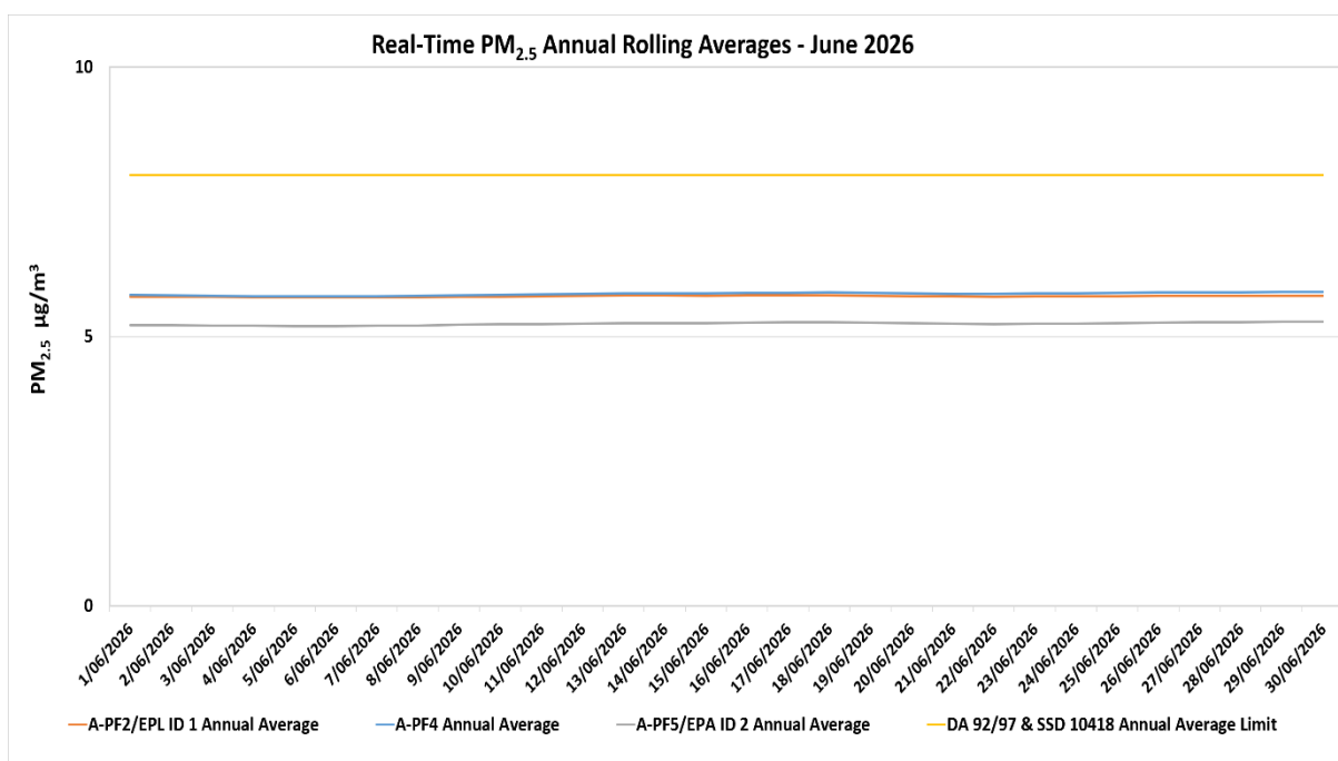
Figure 6-4: Real-time PM 2.5 Annual Rolling Average Results for June 2026.
