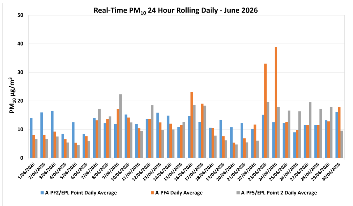
Figure 6-1: Real-time PM 10 24- hourly Daily Average Results for June 2026.
