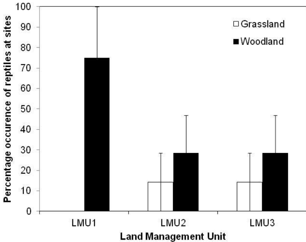
Figure 3.11 Occurrence of reptiles across habitat types at different land management units
