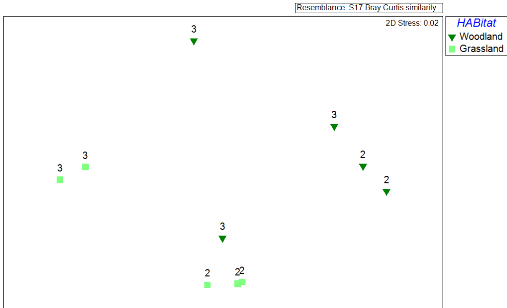
Figure 3.14 MDS plot of MNES monitoring sites at Merriwa West. Colour indicates habitat type and number indicates LMU.
