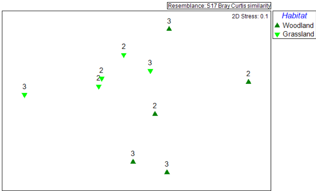
Figure 3.17 MDS plot using flora assemblage at Merriwa West BMA showing LMU class (number) and habitat type (symbols)
