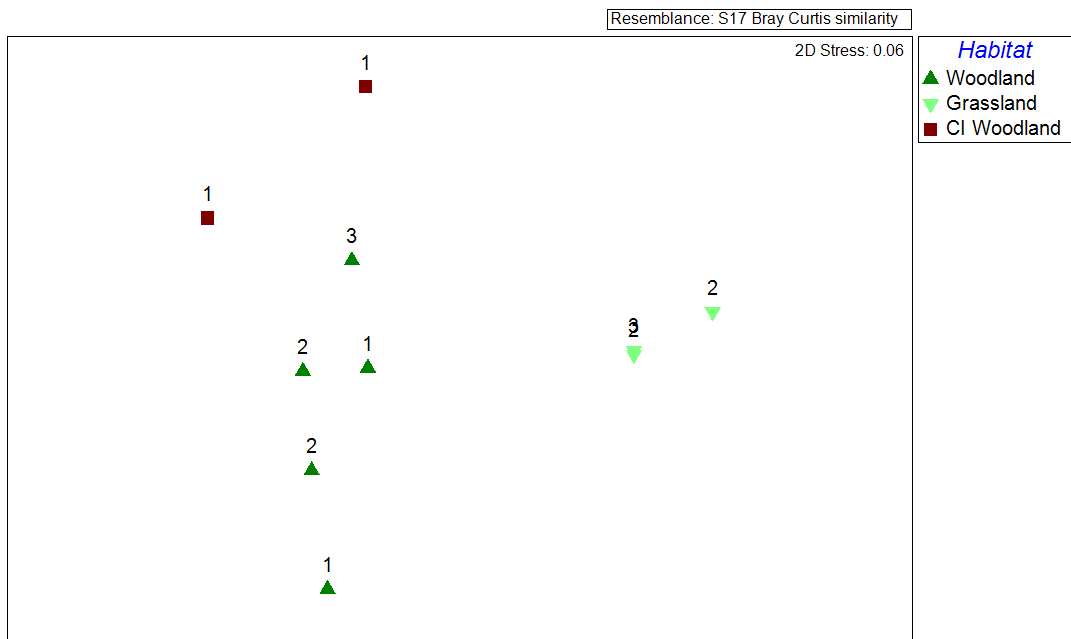
Figure 3.5 MDS plot of habitat features at Namoi BMA showing spread of LMU classes (numbers) and habitats (symbols)
