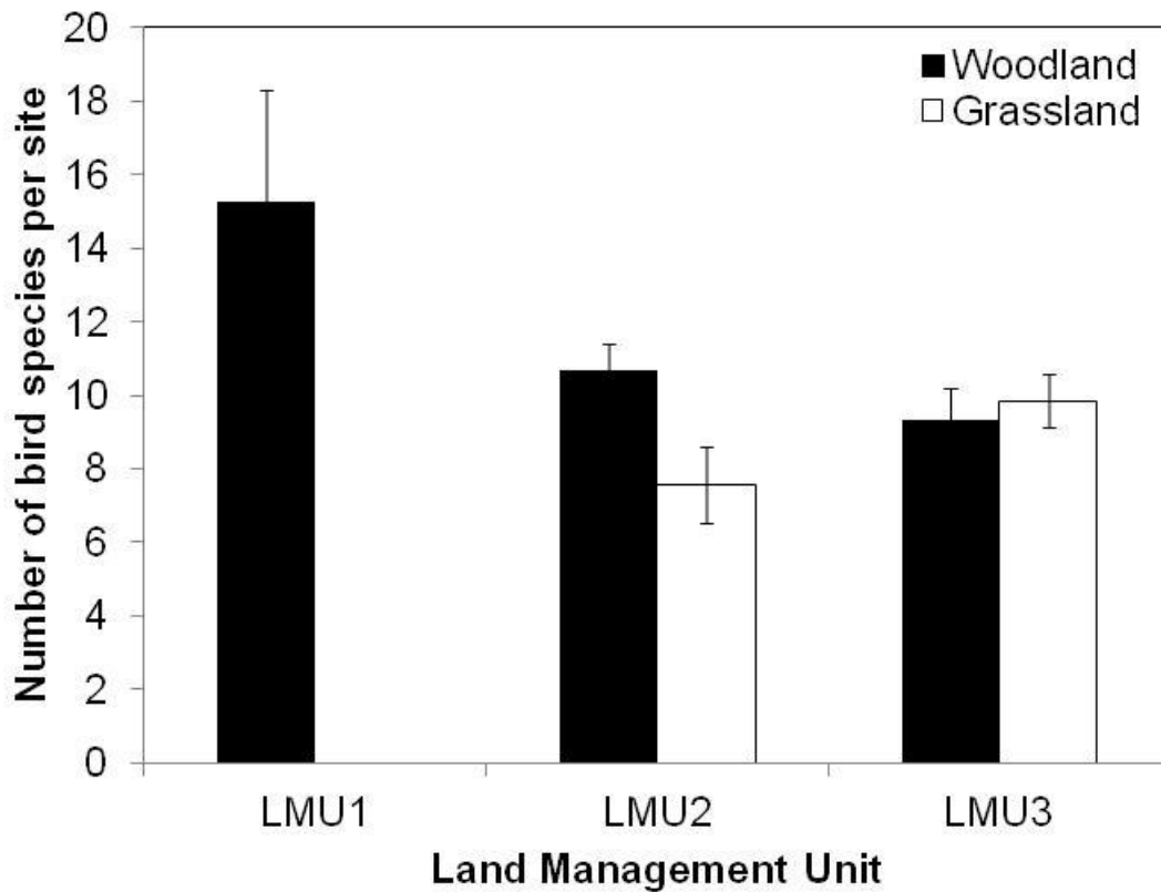
Figure 3.6 Species richness of birds at Indicators of Ecosystem Condition monitoring sites. The above data excludes bird data from riparian sites
