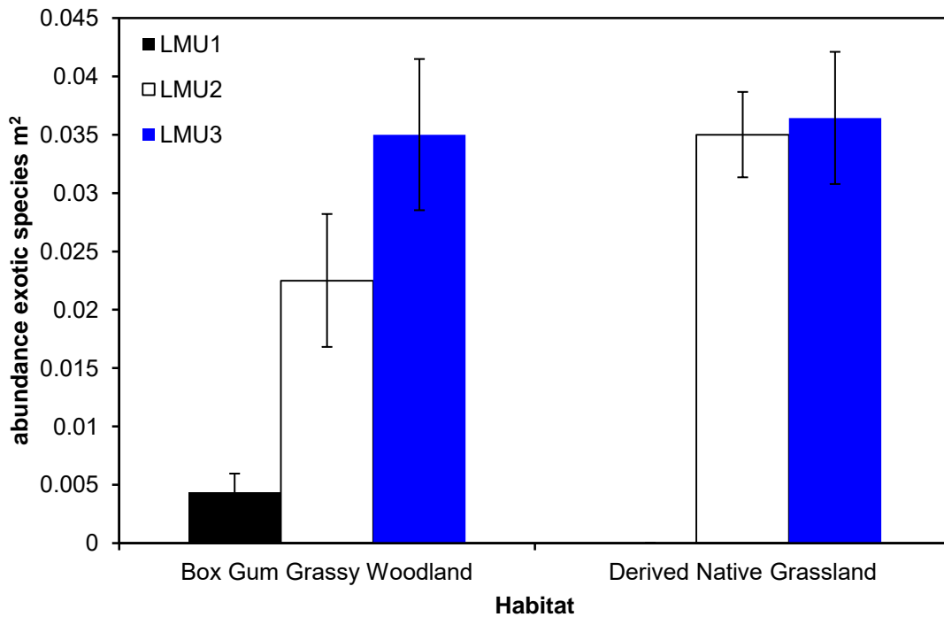
Figure 3.12 Mean number of exotic species m 2 in MNES monitoring plots between habitat types and LMU classes.
