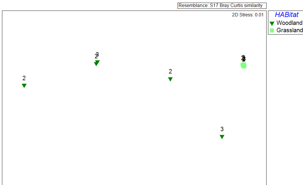
Figure 3.13 MDS plot of MNES monitoring sites at Merriwa East. Colour indicates habitat type and number indicates LMU.
