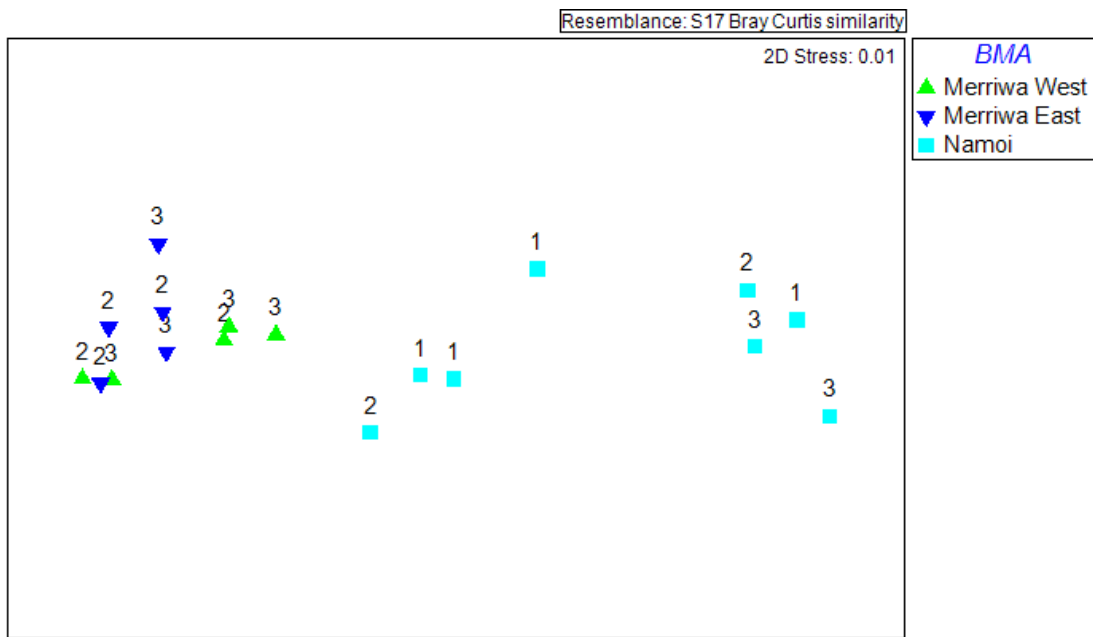
Figure 3.21 MDS plot of soil analysis for Box Gum Grassy Woodland Sites only between BMA (symbol) and LMU (number)
