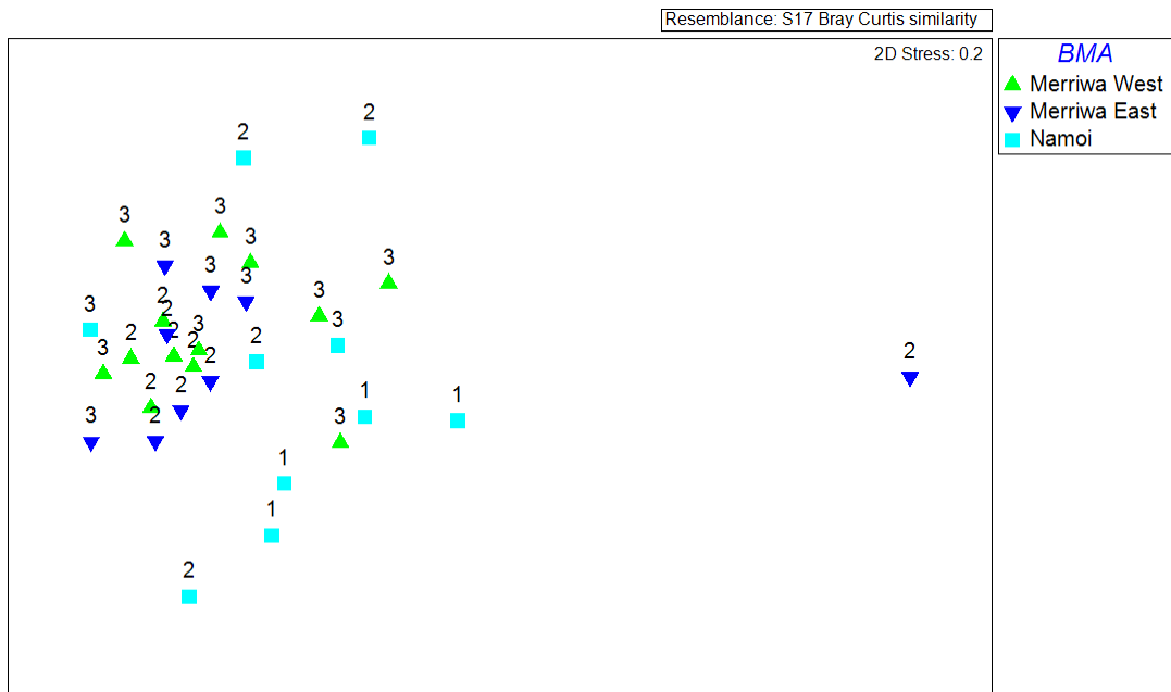
Figure 3.7 MDS plot of bird observations across all BMAs. The colour denotes the BMA and the numbers indicate LMU.
