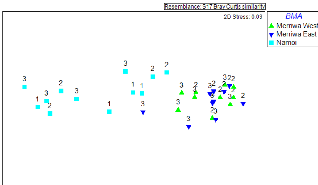
Figure 3.19 MDS plot using soil characteristics between biodiversity management areas (symbols) and land management units (numbers)
