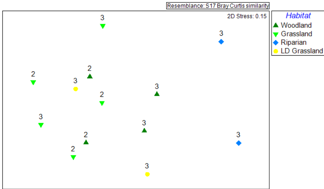
Figure 3.9 MDS Plot of bird observations across LMU classes (numbers) and habitat types (symbols) at Merriwa West BMA
