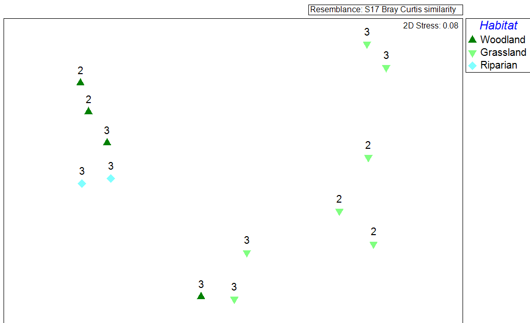
Figure 3.4 MDS plot of habitat features at Merriwa West BMA showing spread of LMU classes (numbers) and habitats (symbols)
