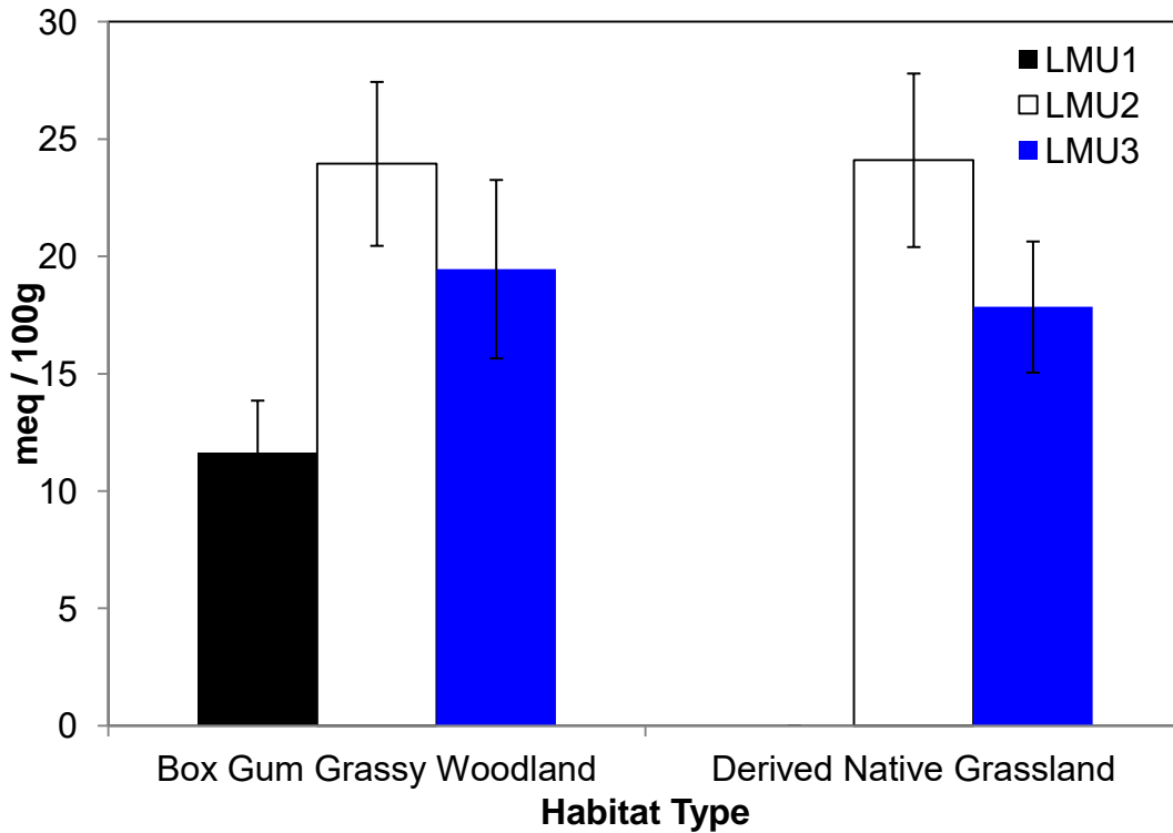
Figure 3.22 Exchangeable calcium at monitoring sites (molar equivalent 100g -1 ) across habitat type and LMU class
