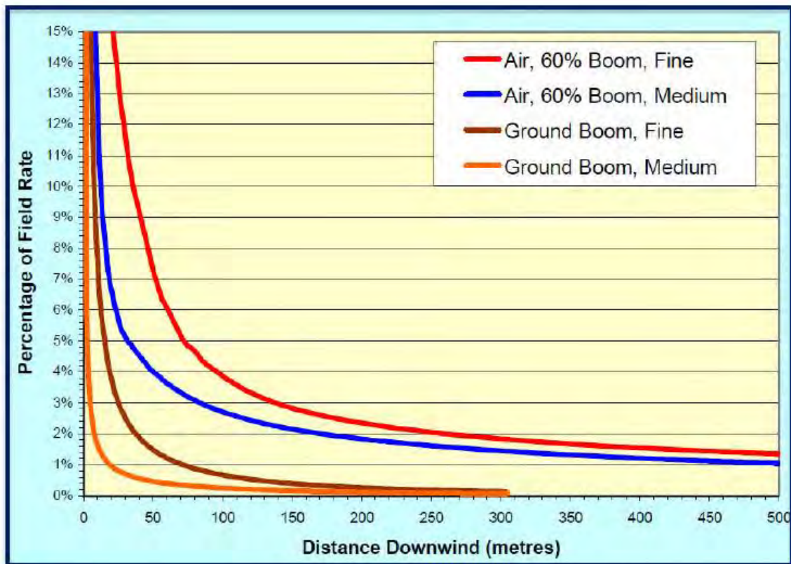
Figure 10 Example of Spray Drift Deposit Profiles from Computer Modelling (APVMA, 2008)
