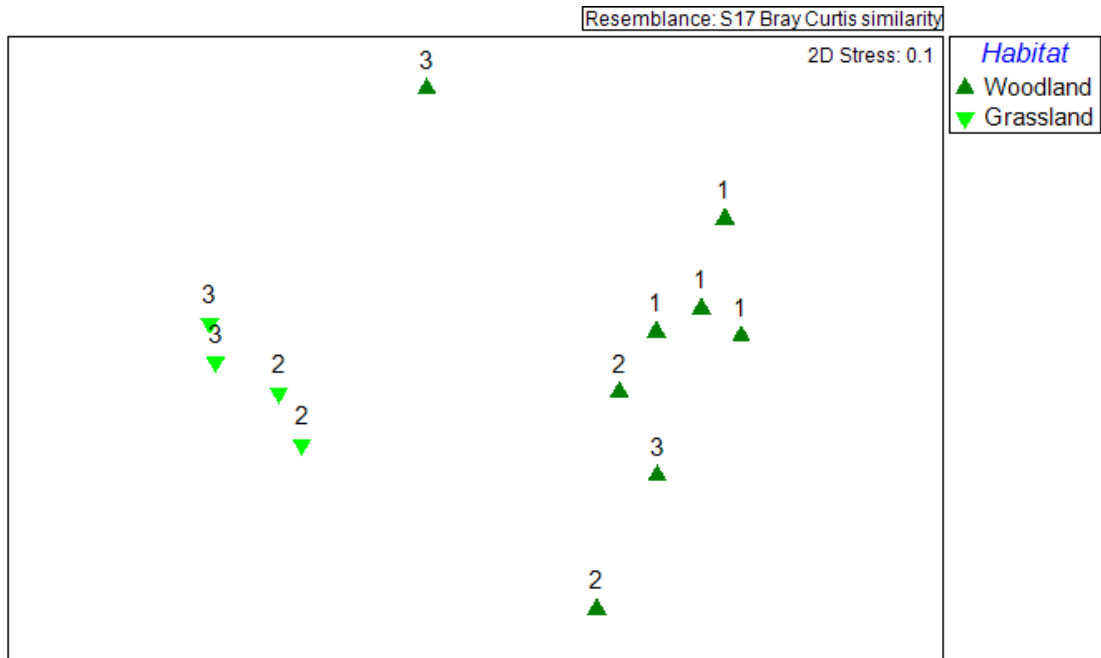
Figure 3.18 MDS plot using flora assemblage at Namoi BMA showing LMU class (number) and habitat type (symbols)
