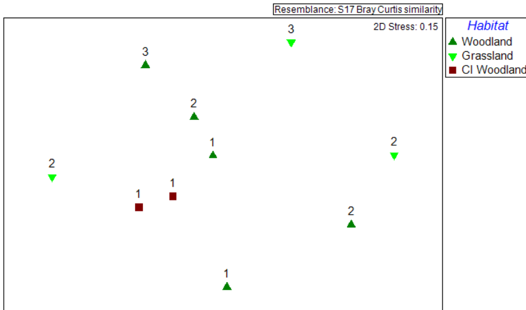
Figure 3.10 MDS Plot of bird observations across LMU classes (numbers) and habitat types (symbols) at Namoi BMA
