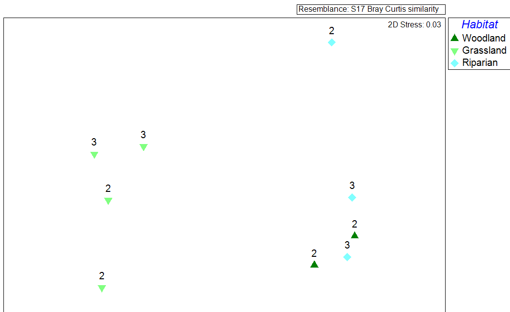
Figure 3.3 MDS plot of habitat features at Merriwa East BMA showing spread of LMU classes (numbers) and habitats (symbols)
