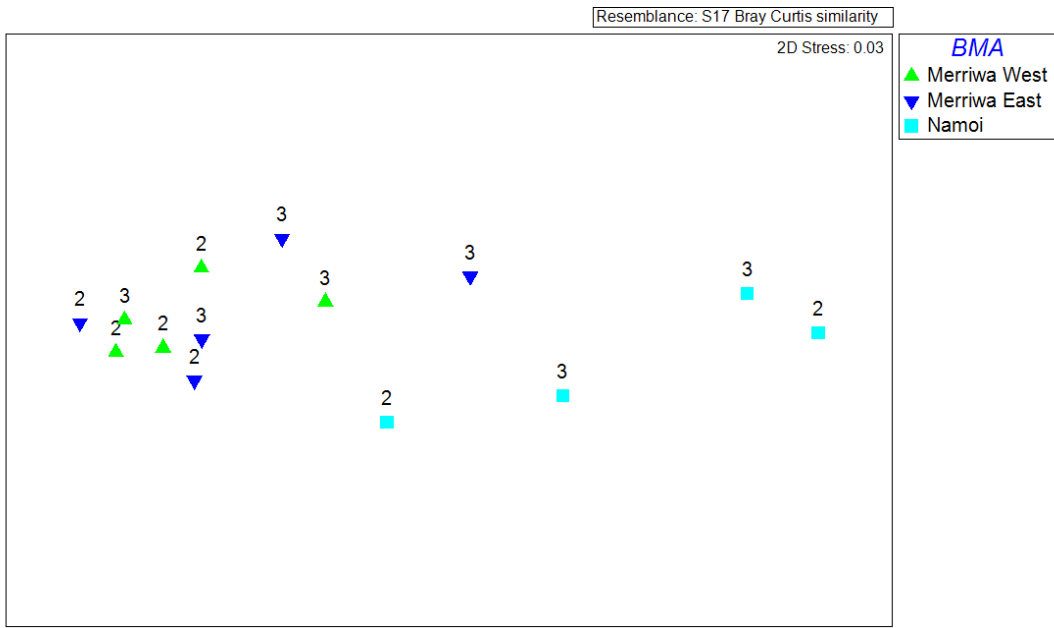
Figure 3.20 MDS plot of soil analysis for Derived Native Grassland Sites only between BMA (symbol) and LMU (number)
