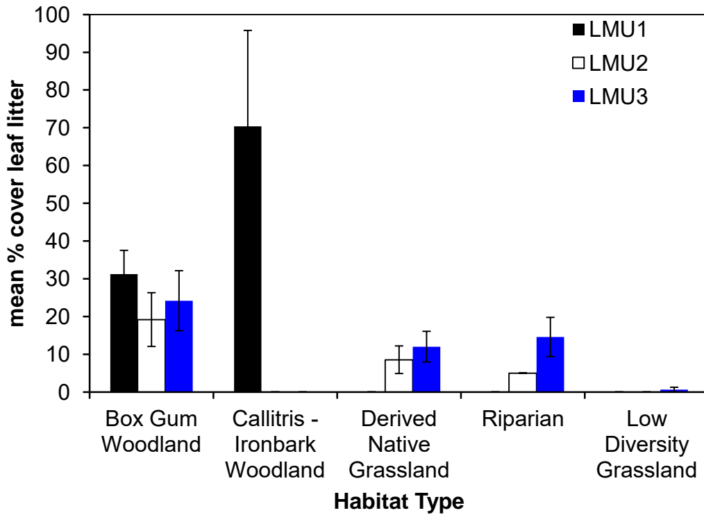
Figure 3.1 Mean percent cover of leaf litter at IEC monitoring sites
