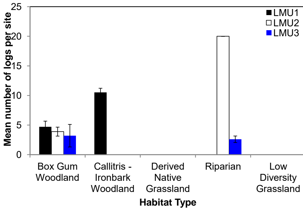
Figure 3.2 Mean number of logs per IEC monitoring site
