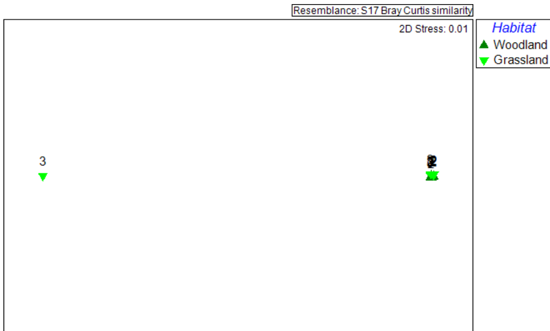
Figure 3.16 MDS plot using flora assemblage at Merriwa East BMA showing LMU class (number) and habitat type (symbols)
