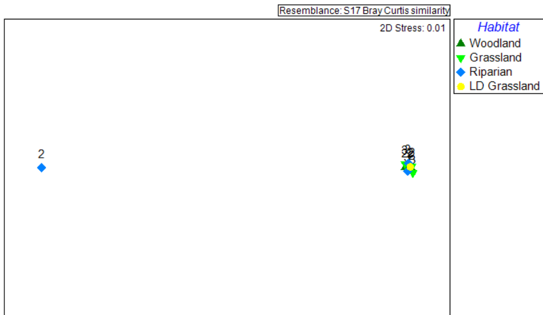
Figure 3.8 MDS Plot of bird observations across LMU classes (numbers) and habitat types (symbols) at Merriwa East BMA
